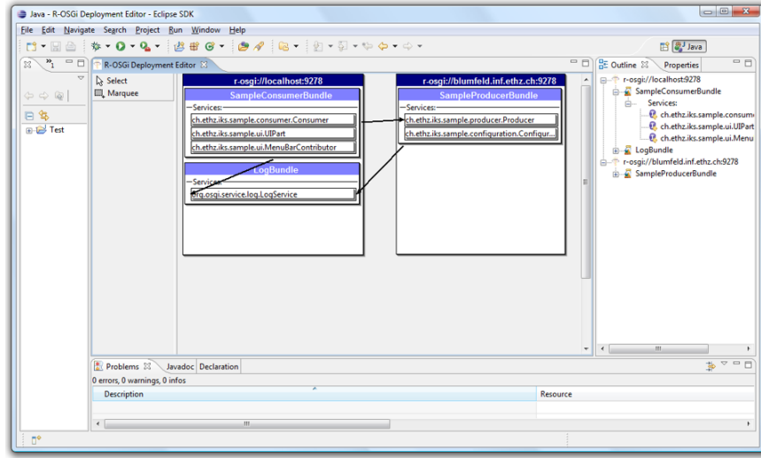
Fig. 5. Screenshot of the R-OSGi Deployment Tool
