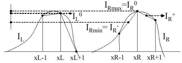
Figure 2: Birchfield's dissimilarity measure: I_{Rmin} \leq I_L^0 \leq I_{Rmax} , thus D_1 equals 0.
