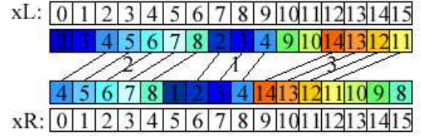
Figure 1: Graphical representation of a match sequence with a left and a right occlusion. The left scanline is on top. The corresponding disparities are also indicated.
