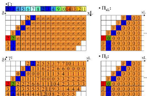
Figure 4: The 4 compressed matrices \Pi_{xL} , \Pi_{\delta} , \gamma and \Gamma . The filling has just started.
