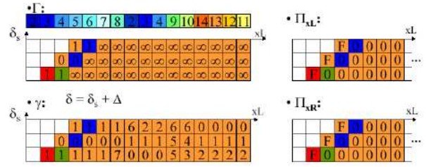
Figure 6: The 4 reduced matrices used in the hierarchical stereo calculation.
