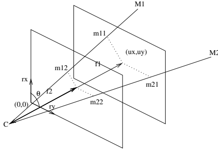
Fig. 1. Illustration of the camera and zoom model. The focal lengths f_1 and f_2 are different, the other parameters ( r_x, r_y, u_x, u_y, \theta ) are identical.
