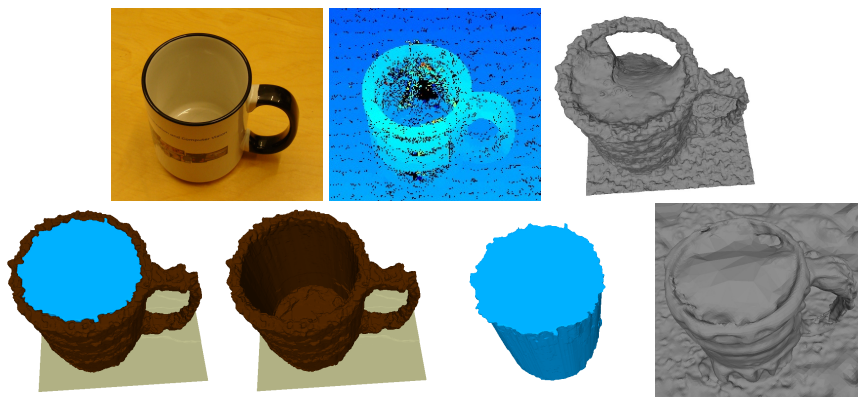
Figure 8. Top row, from left to right: example input image, example depth map, baseline TV-flux fusion result. Bottom row, from left to right: result of our formulation (inner free space inside the mug), result of our shape prior formulation (mug and inner free space separately), PMVS+PSR result.
