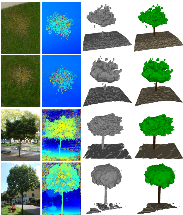
Figure 6. From left to right: Example input image, example depth map, baseline TV-flux fusion result, result using our shape prior formulation.
