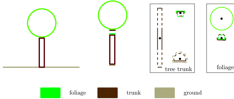
Figure 5. Shape prior formulation for the trees: The tree gets segmented into convex parts (foliage and trunk), the transitions of each part to other labels are taken into account, for each transition the smoothness is defined in terms of Wulff shapes. The dashed lines indicate that the shape is very large in the indicated direction, meaning that this is an unlikely interface in the final reconstruction.
