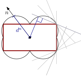
Figure 3. Wulff shape illustration in 2D: The Wulff shape induces an anisotropic smoothness term. The distance from the origin to the black line in direction n is the cost d^n for a normal direction n . The construction is indicated with gray lines. Naturally the reconstructed shape using this prior has the same shape as the Wulff shape.
