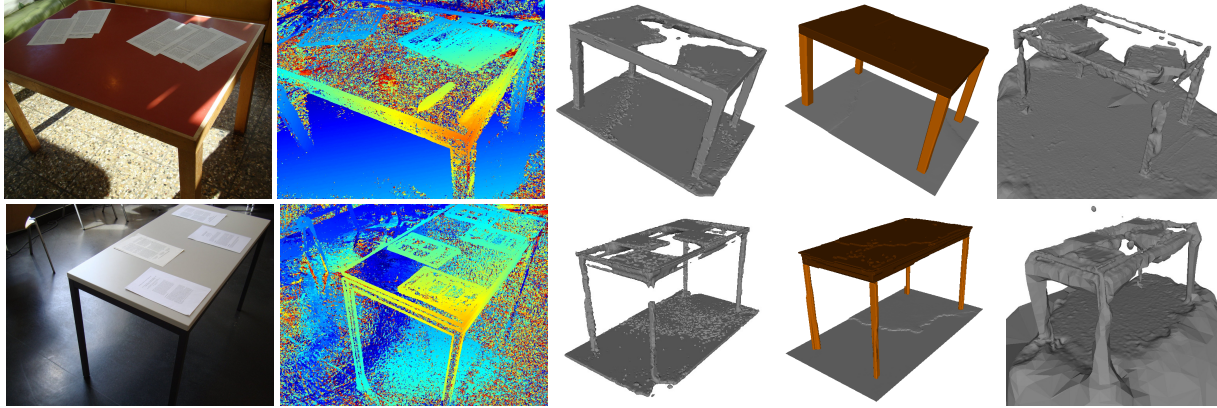
Figure 4. From left to right: example input image, example depth map, baseline TV-flux fusion result, result using our shape prior formulation, PMVS+PSR result.
