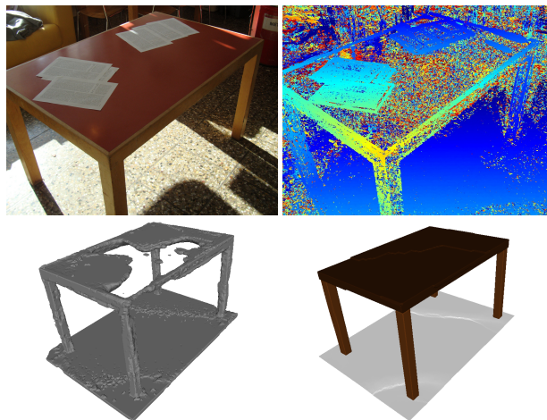
Figure 1. Top: Example input image and depth map. Bottom: Standard volumetric fusion result (left) and our result using the proposed segment based shape prior (right).
