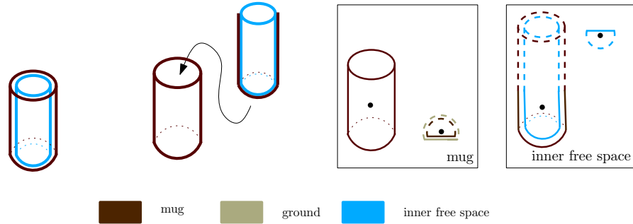
Figure 7. Shape prior formulation for the mug: The mug is segmented as a single convex part (mug) and an interior convex part (inner free space) which gets carved out, the transitions of each part to other labels are taken into account, for each transition the smoothness is defined in terms of Wulff shapes. The dashed lines indicate that the shape is very large in the indicated direction, meaning that this is an unlikely interface in the final reconstruction.
