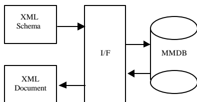
Figure 5 – XML Document
