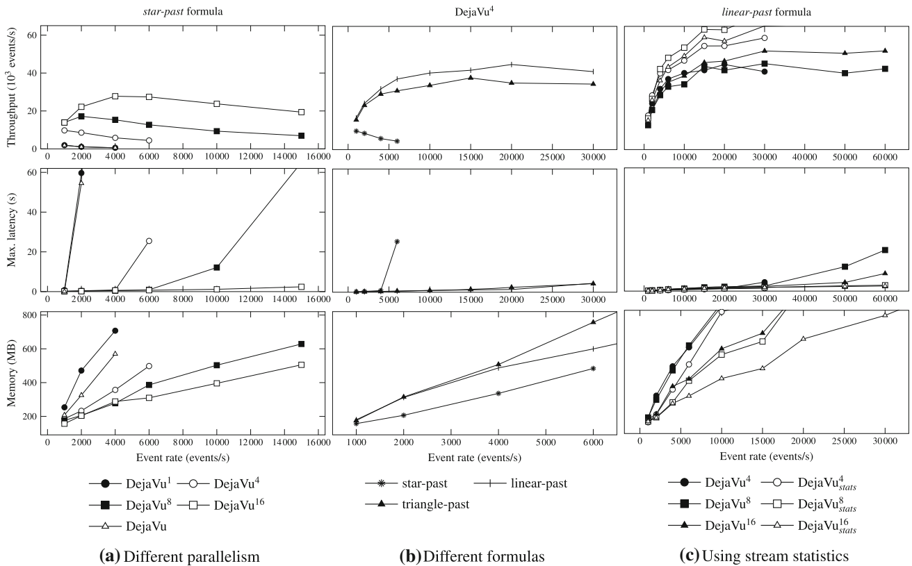
Fig. 8 Synthetic DejaVu experiments: monitoring synthetic streams with DejaVu and without fault tolerance
