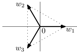
Figure 5: The vectors w_1, \dots, w_r for r = 3 .
