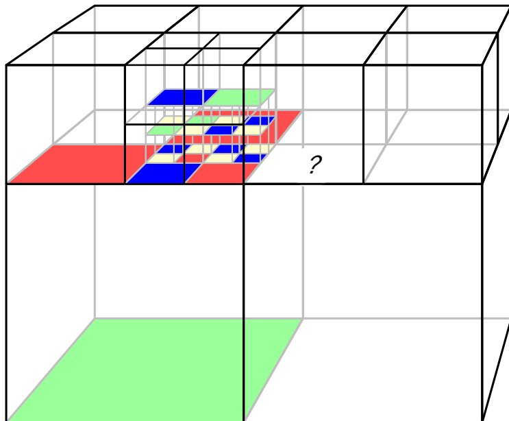
(b) Remaining colors are forced.
