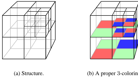
Fig. 1. An octree.
