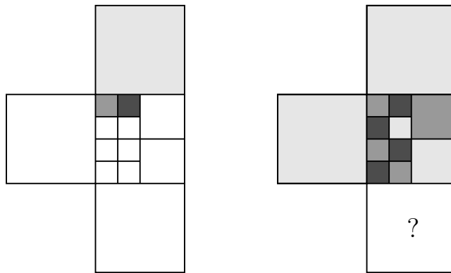
(a) Initial 3-clique. (b) Remaining colors are forced.
