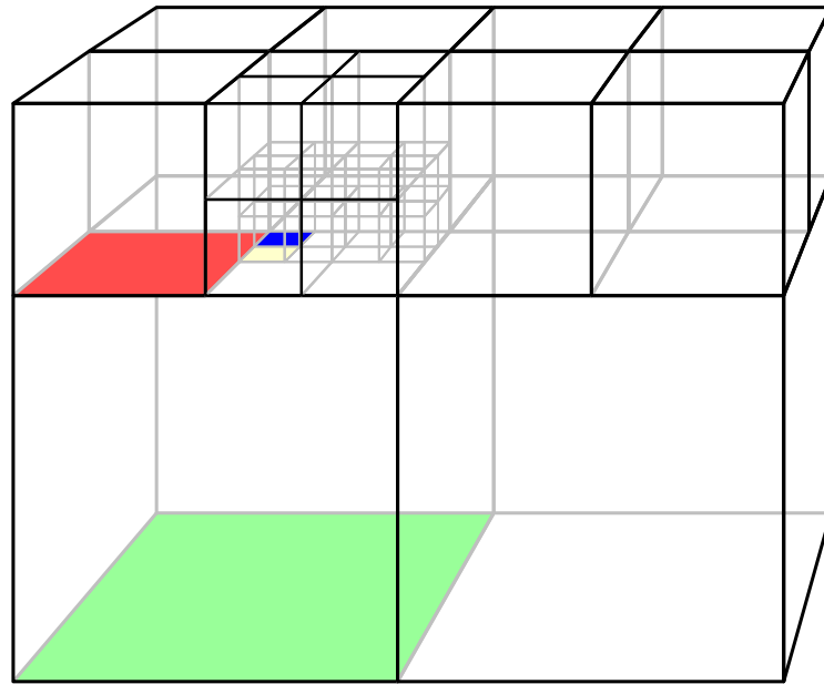
(a) Initial 4-clique.
