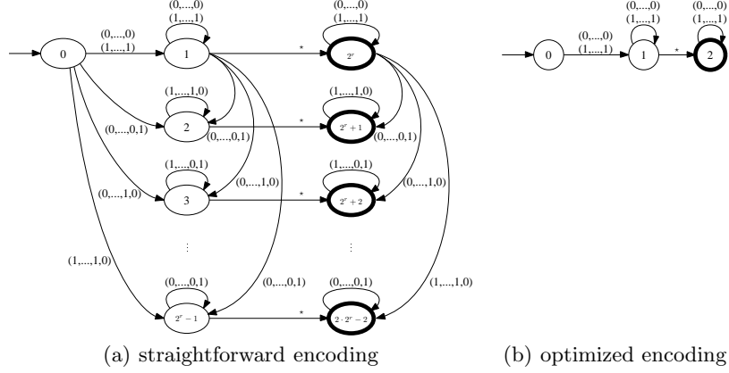
Fig. 2. Minimal WDBAs for the formula \bigwedge_{1 \leq i < r} x_i = x_{i+1} . For the sake of readability, we have omitted the rejecting sink states and their incoming transitions.
